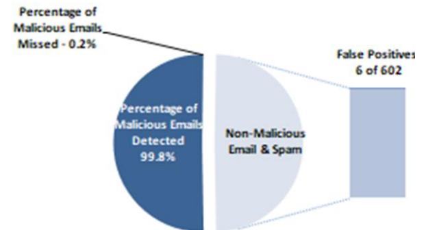
Fig. 2 – 1,224 ATD-Email Test Runs
