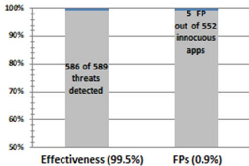
Fig. 1 – 1,141 Standard ATD Test Runs
