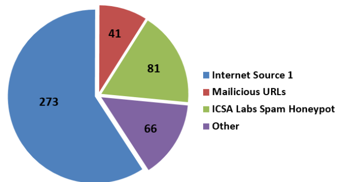
Fig. 12 – Unmodified/Non-Dropped Sample Sources
